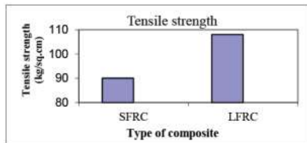
Fig 1.9: Plot of tensile strength v/s type of composite
