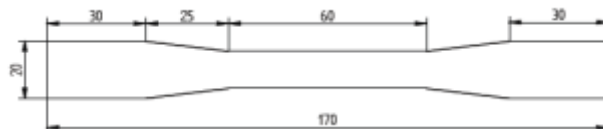
Figure 1.5: Tensile test specimen
