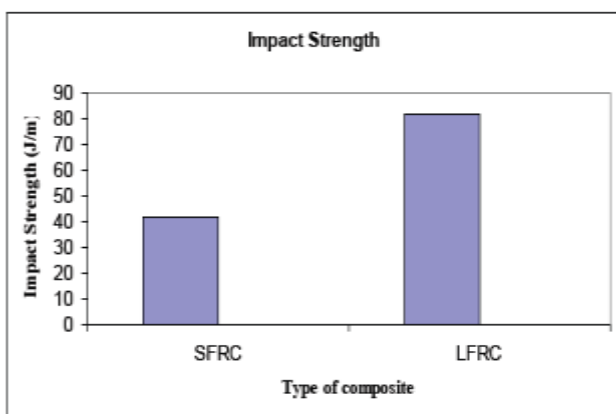
Fig 1.16: Plot of Impact strength v/s type of composite
