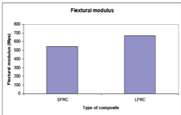
Fig. 1.15: Plot of flexural modulus v/s type of composite
