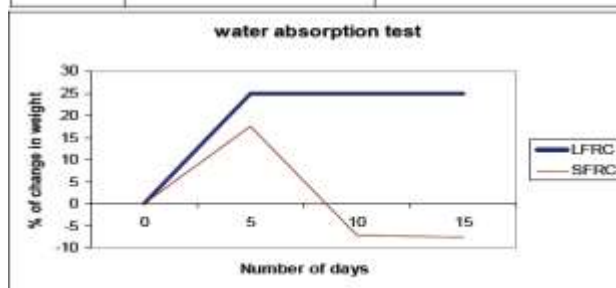
Fig 1.17: Plot of % change in weight v/s number of days
