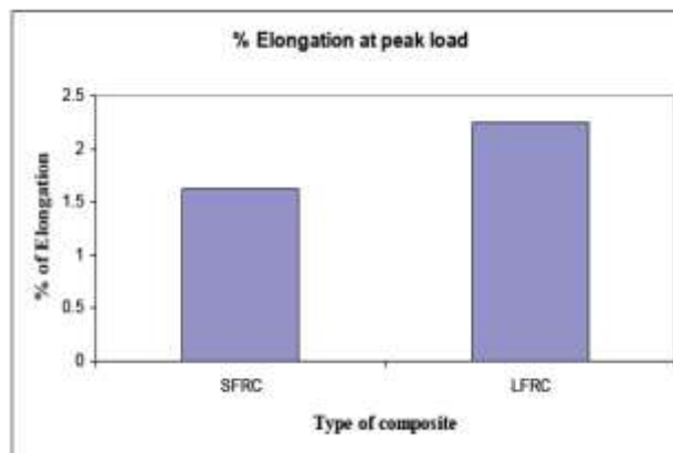
Fig 1.13: Plot of % elongation at peak load v/s type of composite
