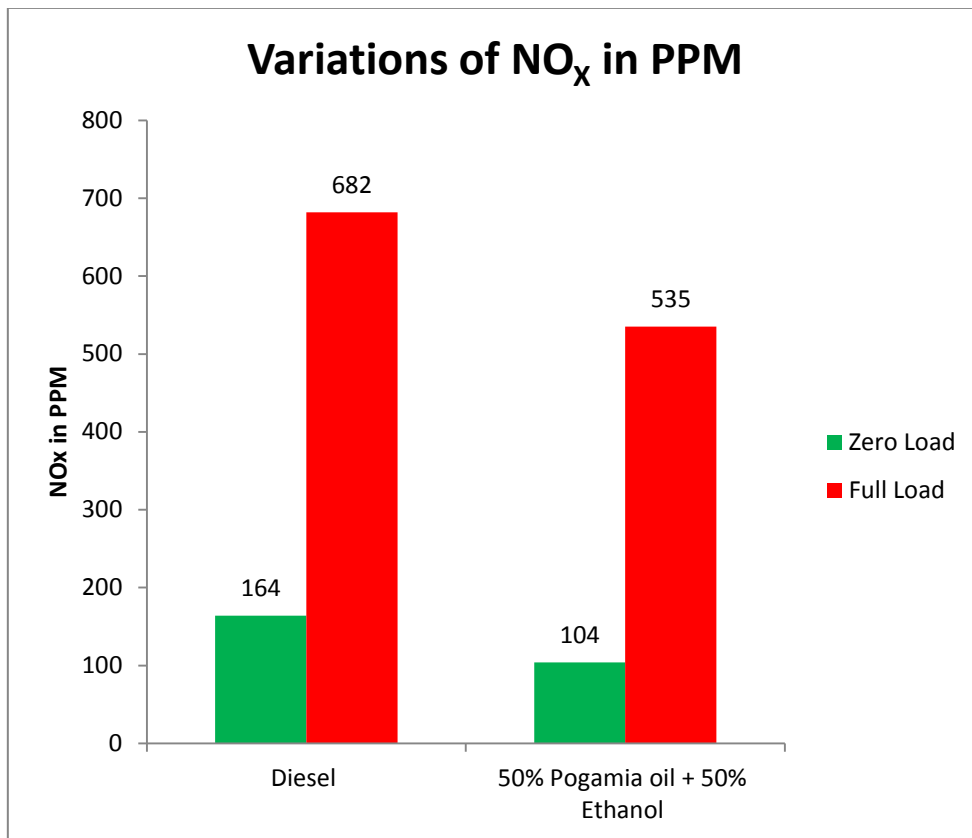
Fig-6 shows the variations of Nitrogen dioxide for Diesel and Pogamia oil blended with Ethanol at Zero Load and Full Load
