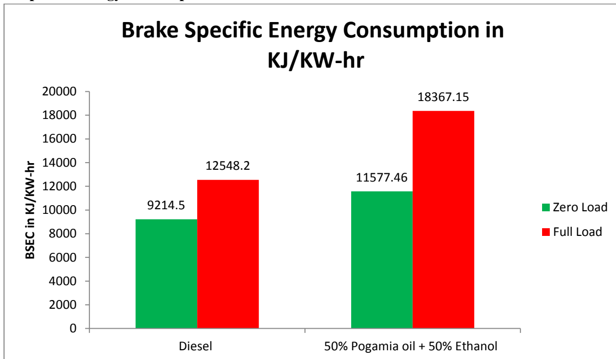
Fig-2 shows the variations of Brake Specific Energy Consumption for Diesel and Pogamia oil blended with Ethanol at Zero Load and Full Load
