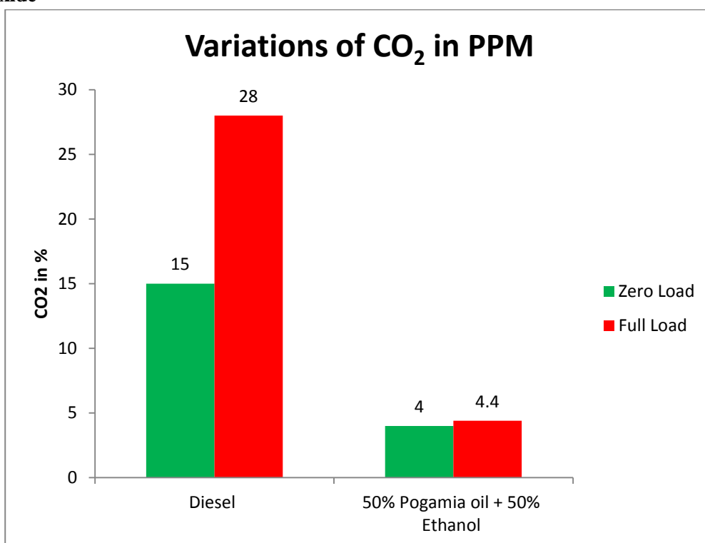
Fig-5 shows the variations of Carbon dioxide for Diesel and Pogamia oil blended with Ethanol at Zero Load and Full Load
