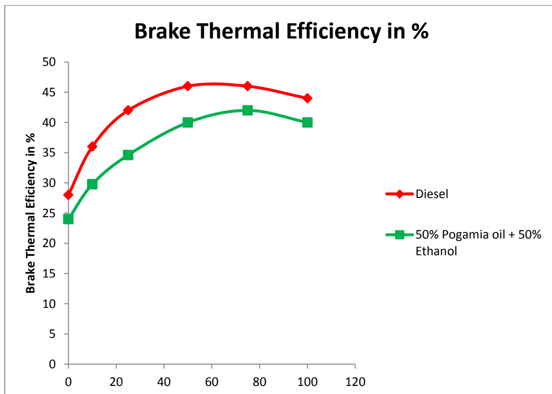
Fig-3 shows the variations of Brake Thermal Efficiency for for Diesel and Pogamia oil blended with Ethanol at different loads
