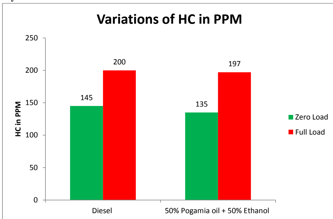
Fig-4 shows the variations of Unburnt Hydro Carbon for Diesel and Pogamia oil blended with Ethanol at Zero Load and Full Load
