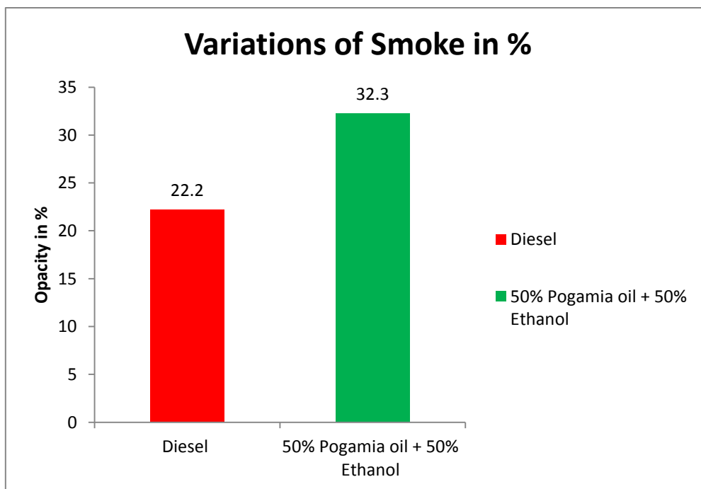
Fig-7 shows the variations of Smoke for Diesel and Pogamia oil blended with Ethanol at Full Load
