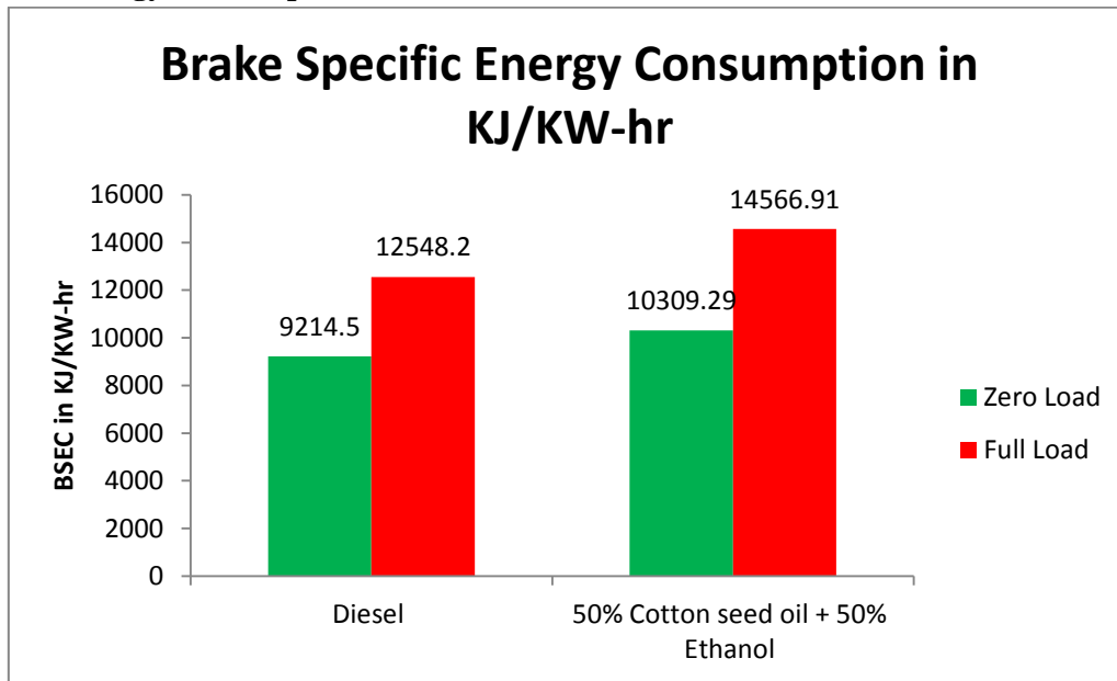
Fig-2 shows the variations of Brake Specific Energy Consumption for Diesel and Cottonseed oil blended with Ethanol at Zero Load and Full Load
