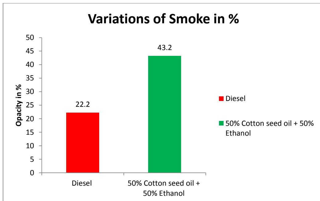
Fig-7 shows the variations of Smoke for Diesel and Cottonseed oil blended with Ethanol at Full Load
