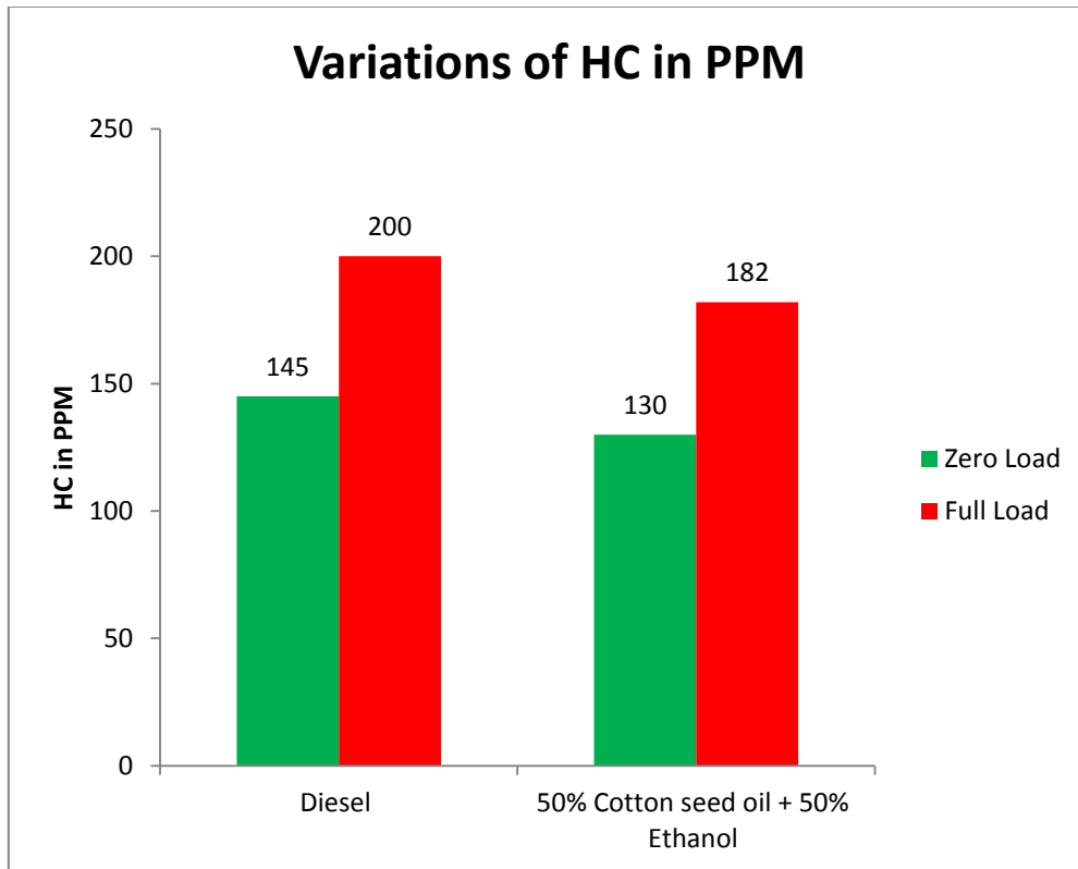
Fig-4 shows the variations of Unburnt Hydro Carbon for Diesel and Cottonseed oil blended with Ethanol at Zero Load and Full Load
