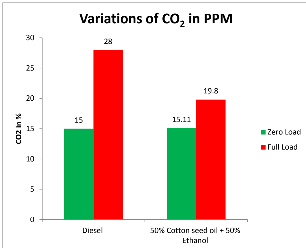
Fig-5 shows the variations of Carbon dioxide for Diesel and Cottonseed oil blended with Ethanol at Zero Load and Full Load
