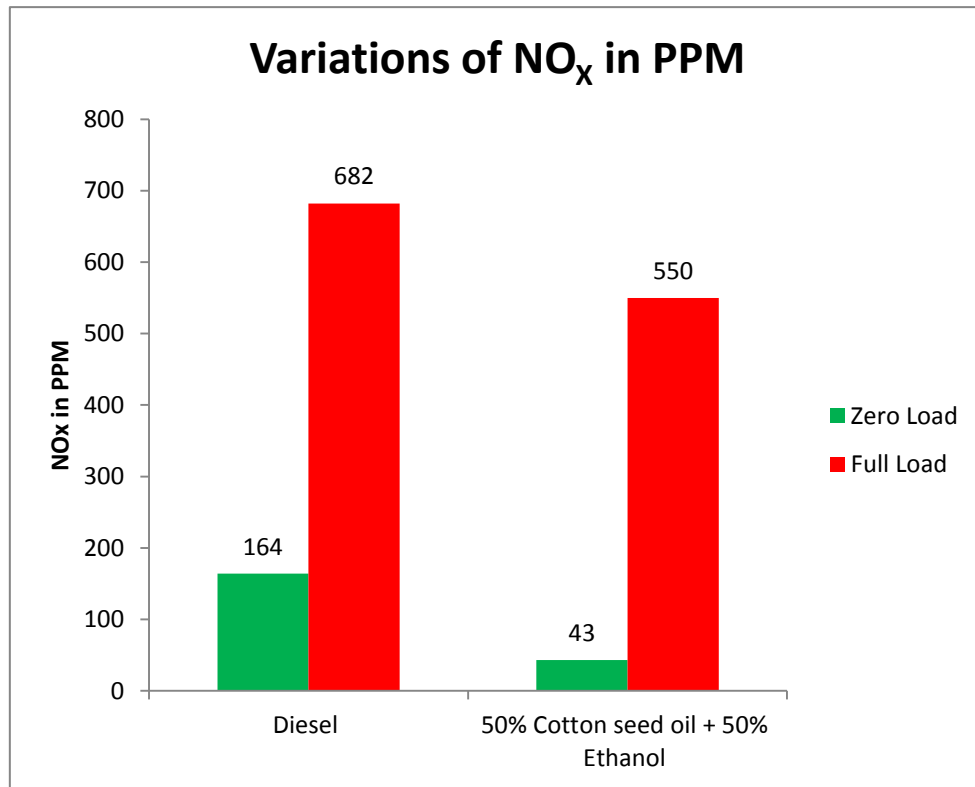
Fig-6 shows the variations of Nitrogen dioxide for Diesel and Cottonseed oil blended with Ethanol at Zero Load and Full Load
