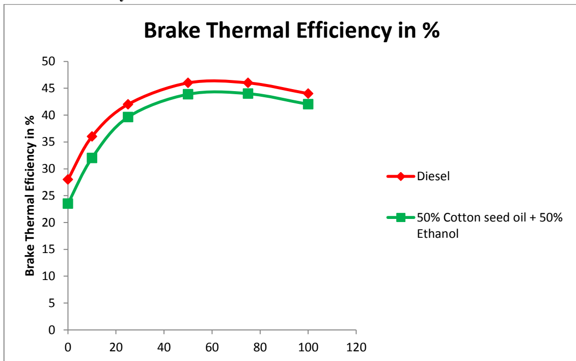
Fig-3 shows the variations of Brake Thermal Efficiency for Diesel and Cottonseed oil blended with Ethanol at different loads
