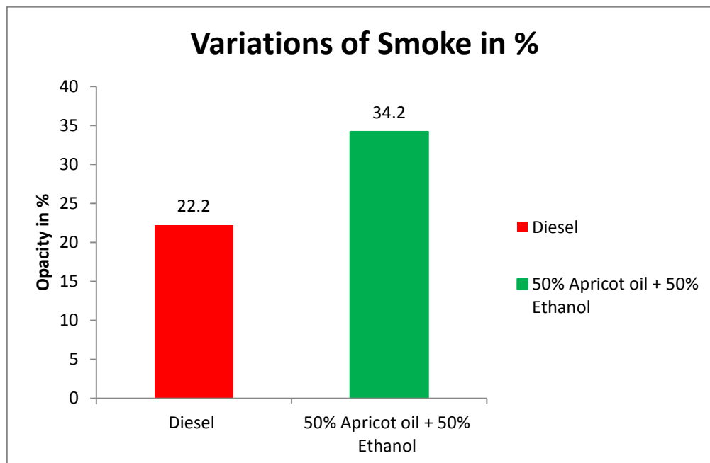
Fig-7 shows the variations of Smoke for Diesel and Apricot oil blended with Ethanol at Full Load
