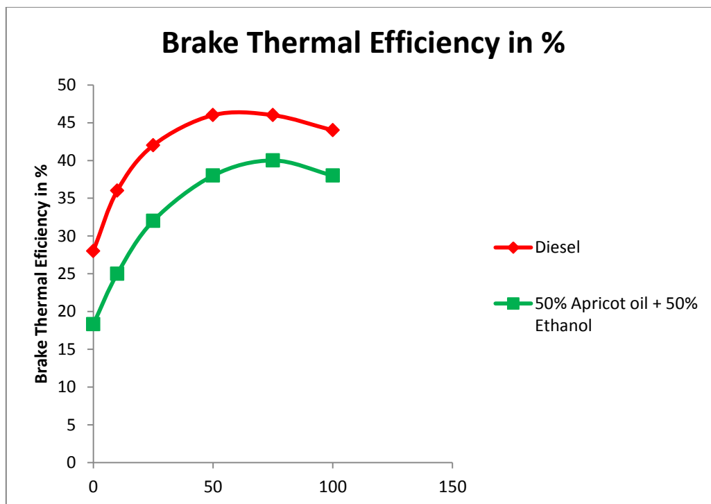
Fig-3 shows the variations of Brake Thermal Efficiency for Diesel and Apricot oil blended with Ethanol at different loads
