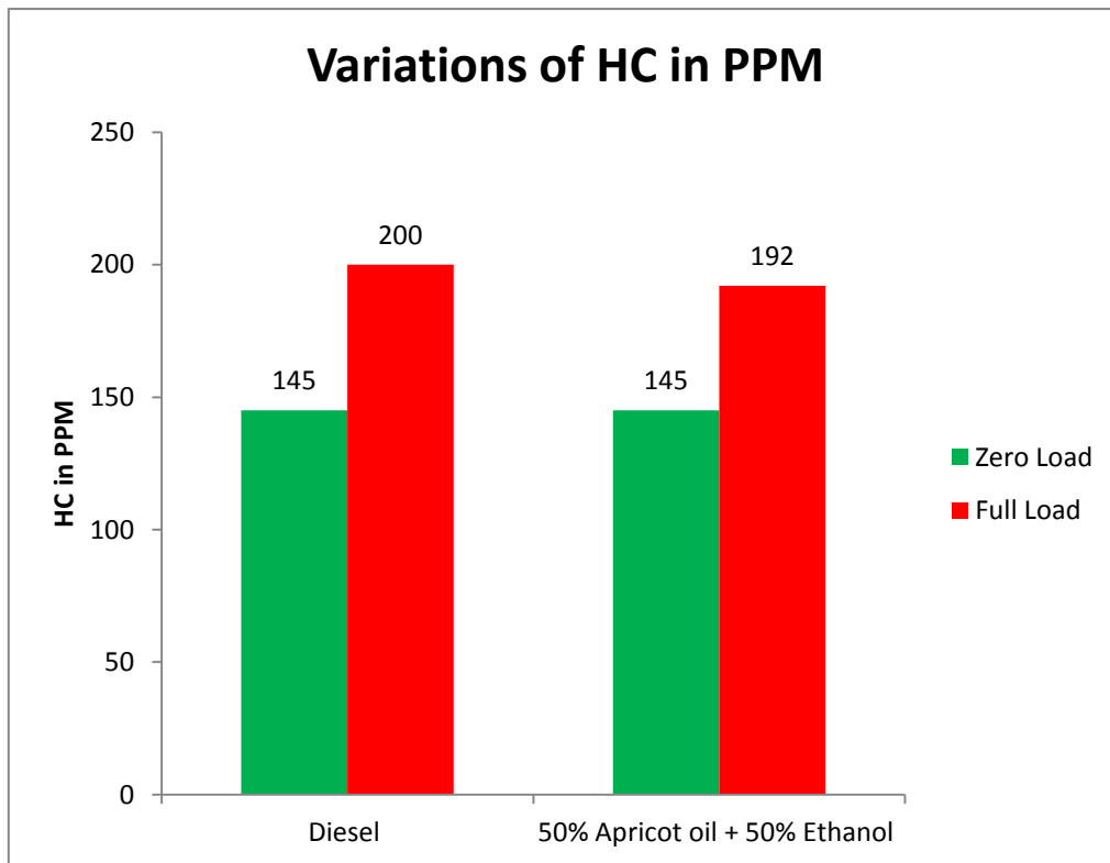
Fig-4 shows the variations of Unburnt Hydro Carbon for Diesel and Apricot oil blended with Ethanol at Zero Load and Full Load
