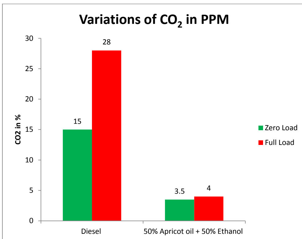
Fig-5 shows the variations of Carbon dioxide for Diesel and Apricot oil blended with Ethanol at Zero Load and Full Load
