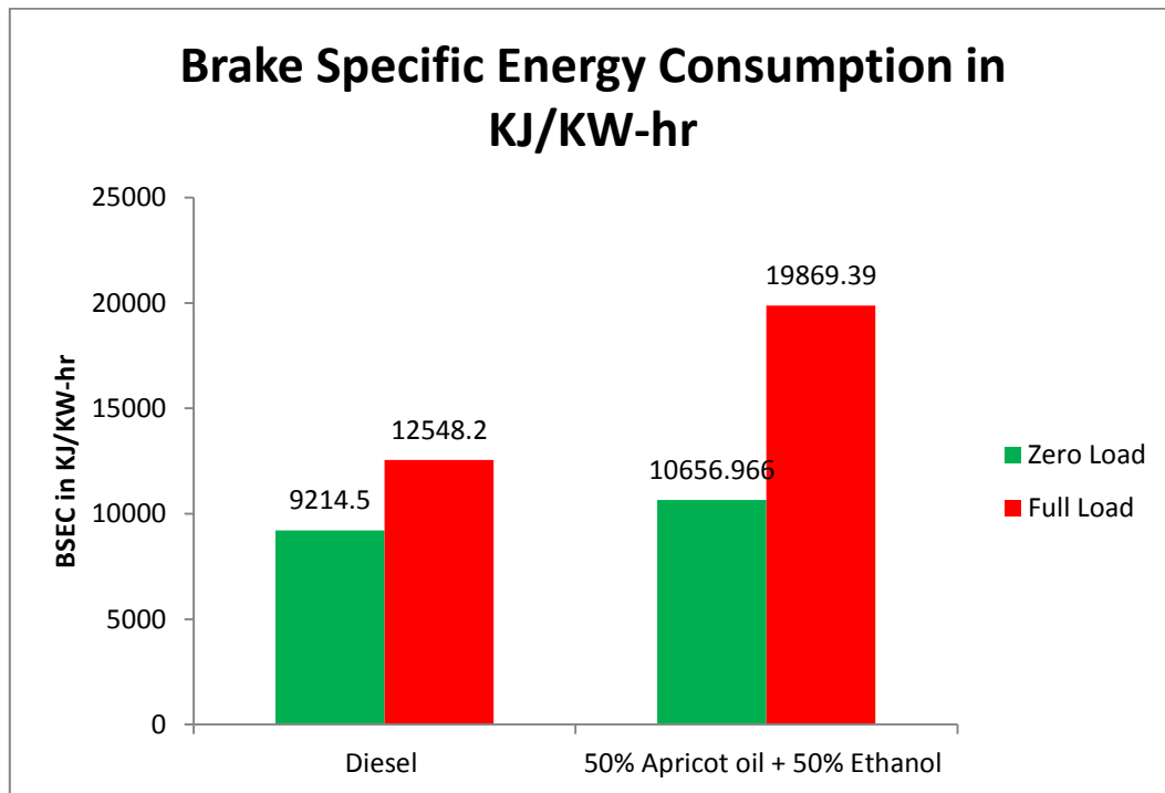
Fig-2 shows the variations of Brake Specific Energy Consumption for Diesel and Apricot oil blended with Ethanol at Zero Load and Full Load
