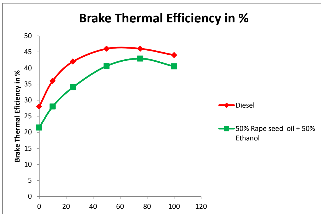
Fig-3 shows the variations of Brake Thermal Efficiency for Diesel and Rape seed oil blended with Ethanol at different loads
