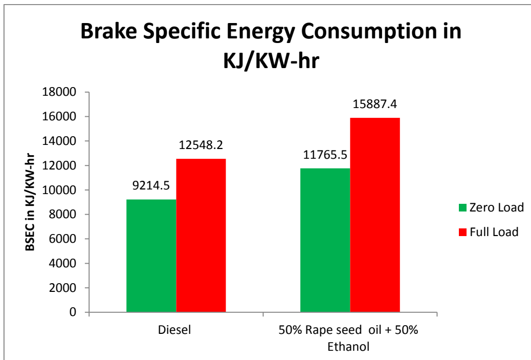
Fig-2 shows the variations of Brake Specific Energy Consumption for Diesel and Rape seed oil blended with Ethanol at Zero Load and Full Load
