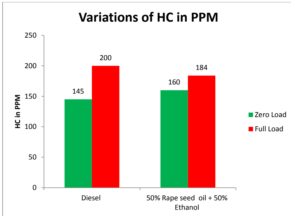
Fig-4 shows the variations of Unburnt Hydro Carbon for Diesel and Rape seed oil blended with Ethanol at Zero Load and Full Load
