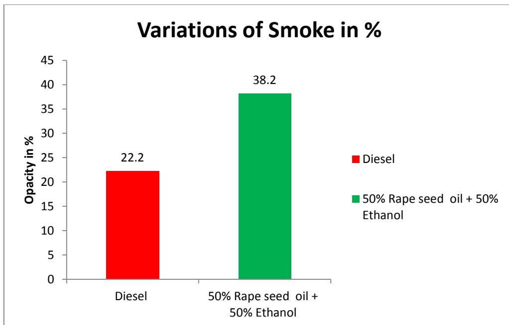
Fig-7 shows the variations of Smoke for Diesel and Rape seed oil blended with Ethanol at Full Load
