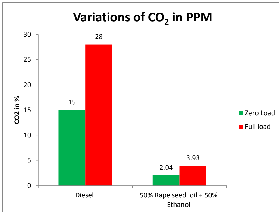
Fig-5 shows the variations of Carbon dioxide for Diesel and Rape seed oil blended with Ethanol at Zero Load and Full Load
